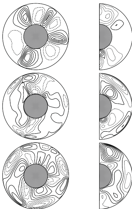
Fig. 3. For the same parameters as in Fig. 2. Equatorial section (left column) and axisymmetric part in meridional section of \mathbf{V} . Minimal and maximal values for the first line (-62.0, 128.8) , (-28.0, 31.9) , for the second (-63.2, 34.6) , (-22.3, 31.9) and for the third line (-90.3, 72.7) , (-11.7, 39.9)
