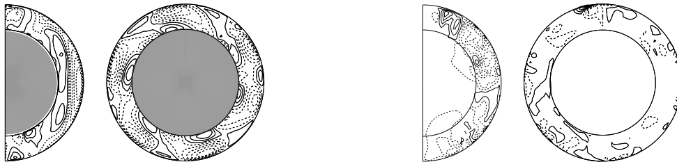
Fig. 7. Regime II, r_{ICB} = 0.67 , E = 3 \cdot 10^{-4} , Pr = 0.1 , Ra = 10^3 , q = 8 on the grid 65 \times 65 \times 64 . Meridional (left column) and equatorial section (right column) of the V_\varphi -component (upper line) and B_\varphi -component (bottom line) of the fields. Minimal and maximal values of the velocity: (-102, 67) , (-112, 62) and magnetic (-0.14, 0.16) , (-1.0, 1.5) fields
