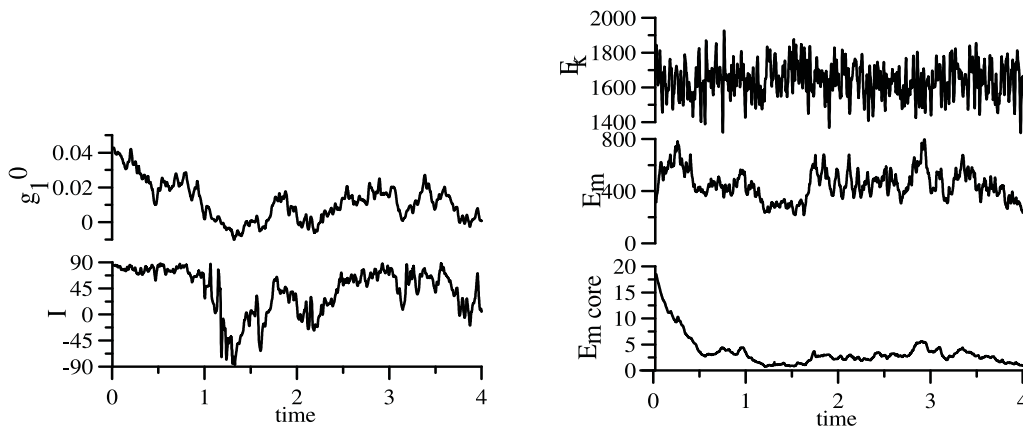
Fig. 8. Regime I, r_{ICB} = 0.67 , E = 10^{-3} , Pr = 1 , Ra = 3 \cdot 10^2 , q = 5 . Evolution of: magnetic dipole g_1^0 , inclination I , kinetic energy E_k , magnetic energy E_m , and magnetic energy of the inner core E_{m\ core}
